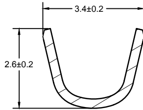
Section view A-A
