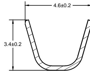
Section view C-C
